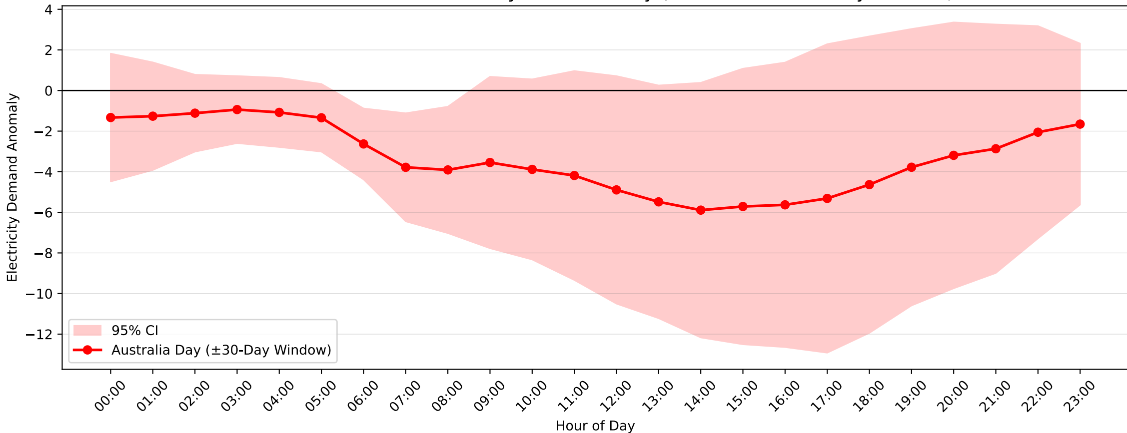
Hunters Hill Demand Anomaly: Australia Day (2016–2017, \pm 30 -Day Window)
